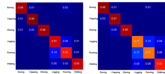
(a) Descriptor-based (b) Prototype-based ( k=220 )
